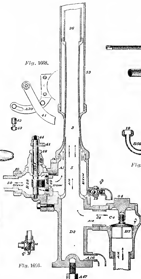
Fig. 1664. Section.
